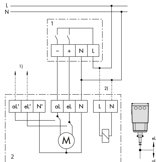
Fig. 11: Electrical connection
