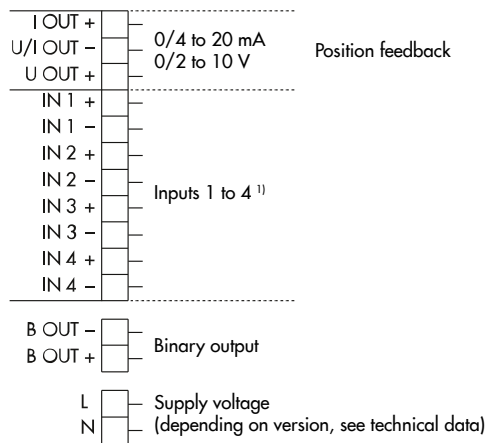
Fig. 14: Electrical connection
